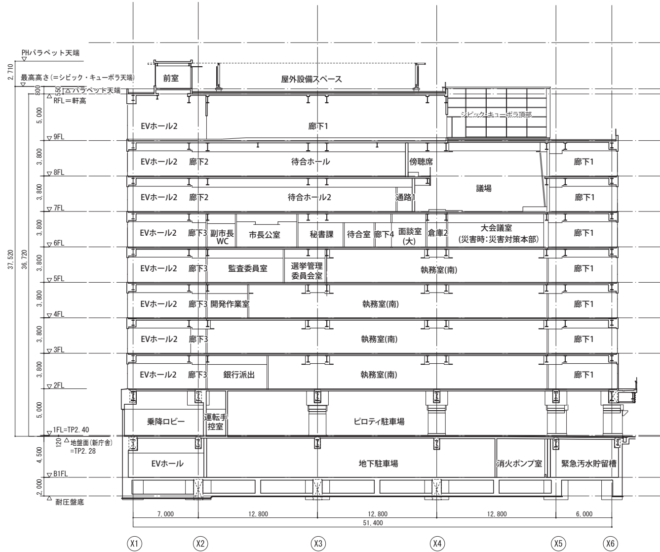
断面図 (Y1a-Y2間)
